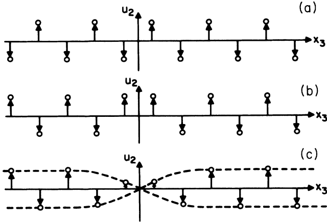
FIG. 3. Alternating displacement pattern along x_2 \parallel [010] of one row of X ions parallel to x_3 passing through an ion at \mathbf{x} = a(\frac{1}{2}, \frac{1}{2}) of Fig. 1(a) for \mathbf{Q} = (0, 0, Q_3) (schematic). (a) Single domain tetragonal phase. (b) Discontinuous (001) antiphase boundary. (c) Continuous (001) antiphase boundary.
